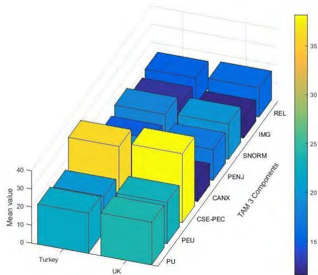
Figure 2. Mean values of the groups based on t-test with the acceptance and usage of CCSs
